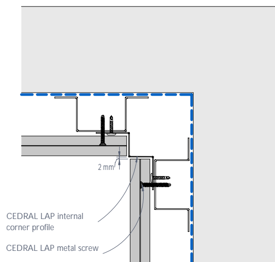
Figure 29: CEDRAL LAP internal corner
