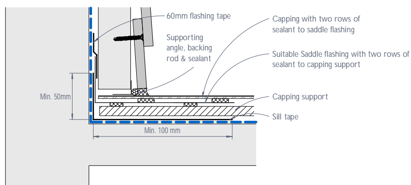
Figure 36: CEDRAL LAP parapet junction - Section
