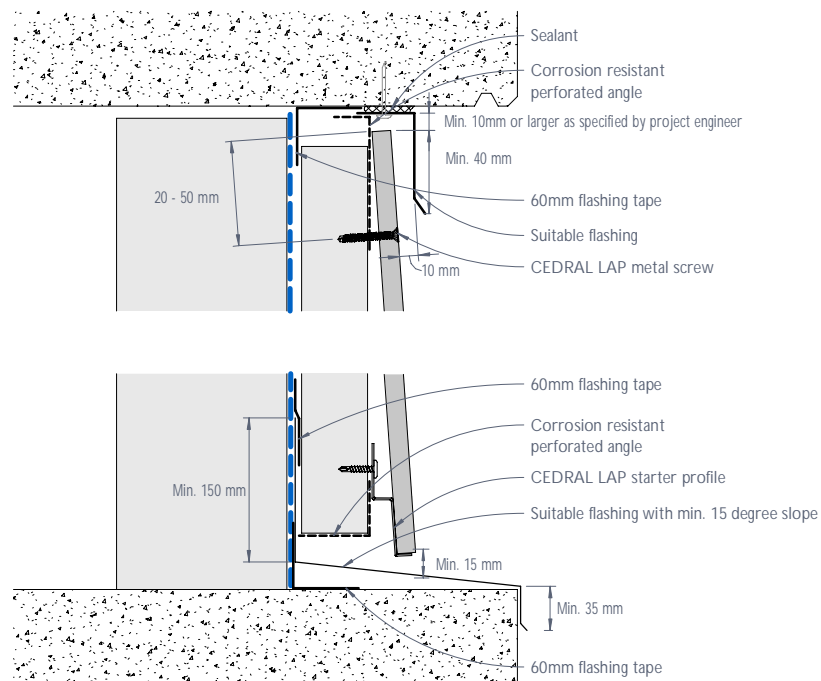
Figure 25: CEDRAL LAP junction with exposed concrete slab or beam - Cladding recessed
