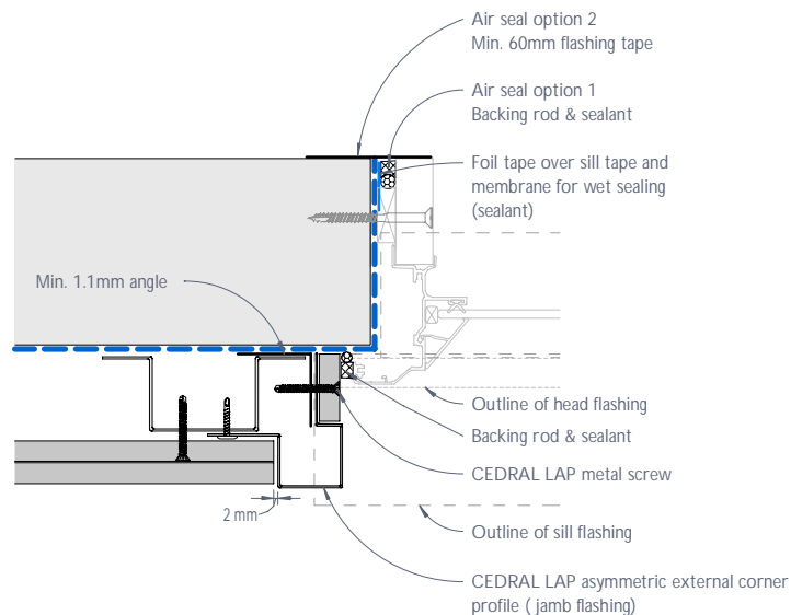
Figure 10: CEDRAL LAP window jamb junction or the like - Detail 1
