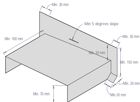
Figure 38: Suitable saddle flashing
