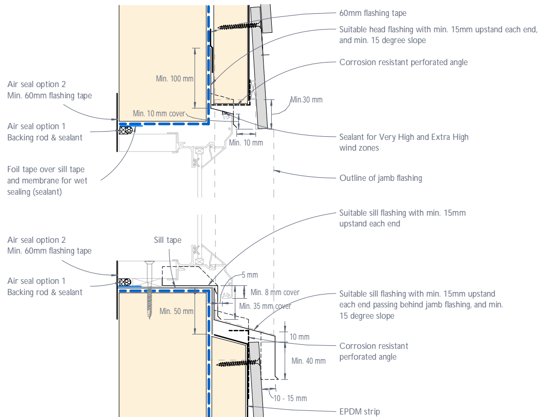
Figure 10: CEDRAL LAP window head and sill junction without CEDRAL starter profile at the head
