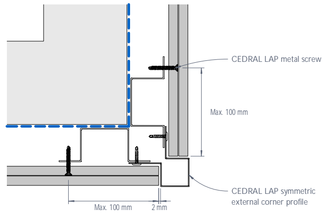
Figure 26: CEDRAL LAP typical external corner
