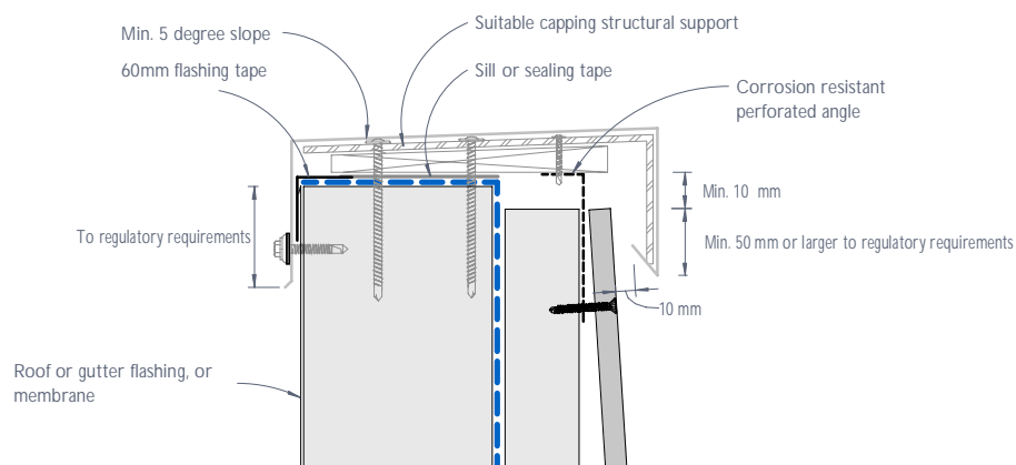
Figure 34: CEDRAL LAP typical capping detail
