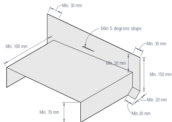
Figure 38: Suitable saddle flashing
