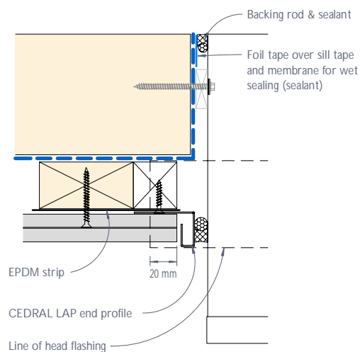
Figure 14: CEDRAL LAP meter box junction - Plan view
