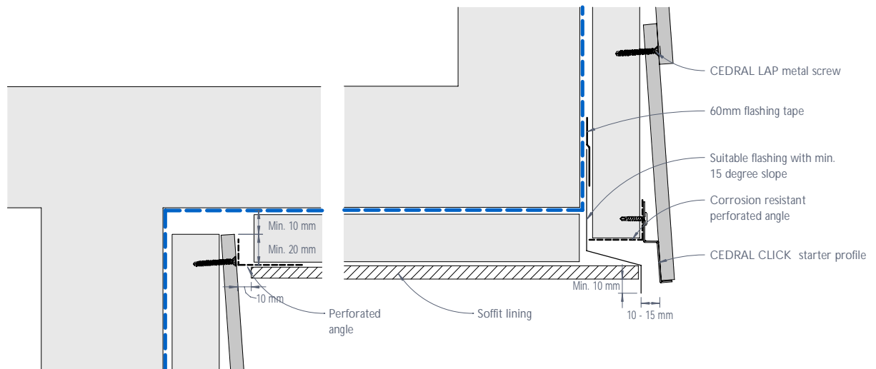
Figure 16: CEDRAL LAP soffit junction
