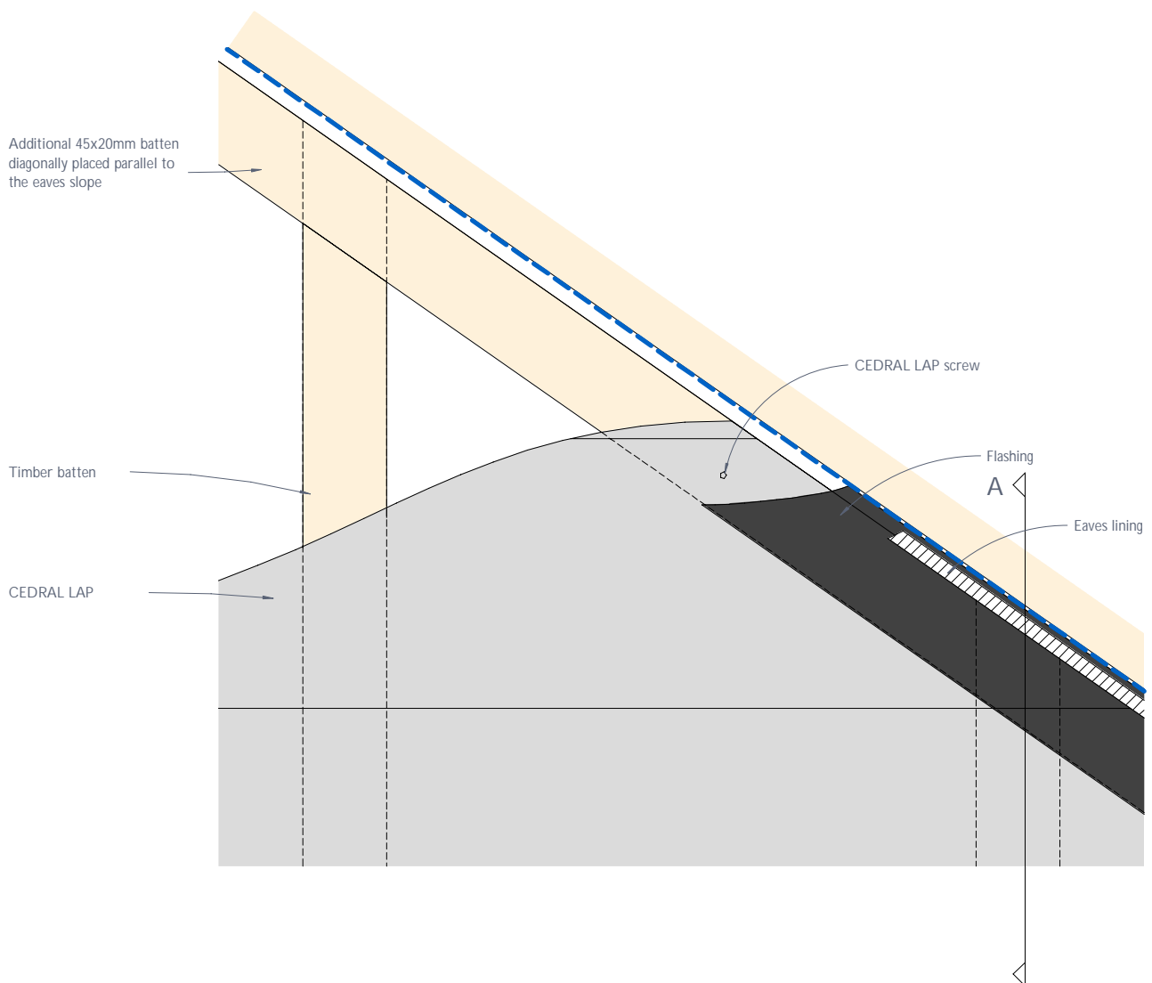
Figure 22: CEDRAL LAP junction with angled eave - Elevation
