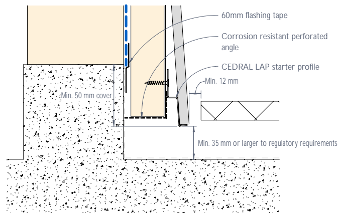
Figure 18: CEDRAL LAP base detail - Covered area
