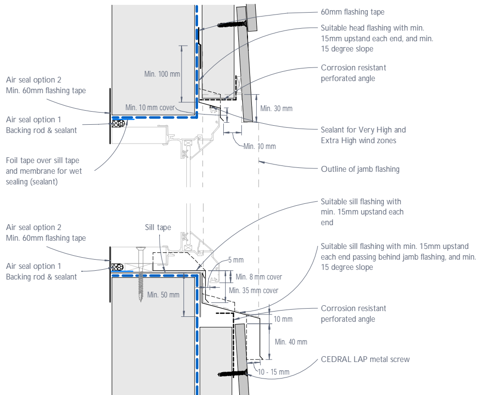
Figure 10: CEDRAL LAP window head and sill junction without CEDRAL starter profile at the head
