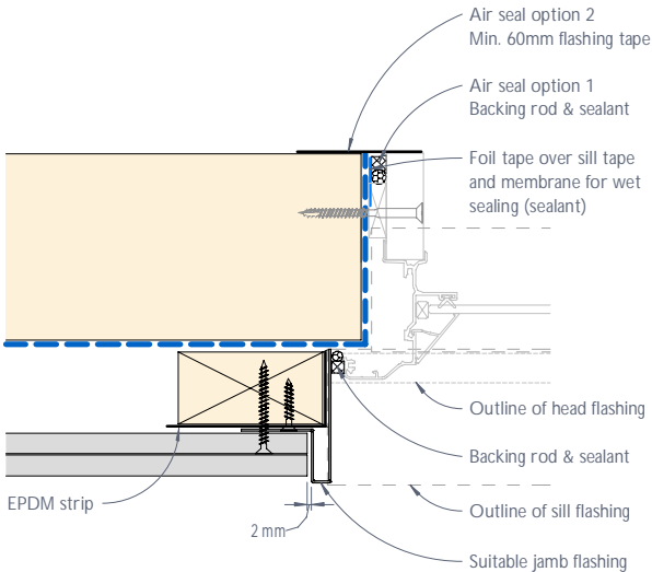
Figure 12: CEDRAL LAP window jamb junction or the like - Detail 3
