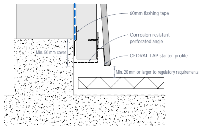
Figure 19: CEDRAL LAP base detail - Balcony
