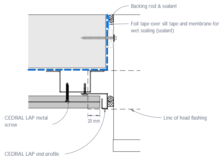
Figure 14: CEDRAL LAP meter box junction - Plan view
