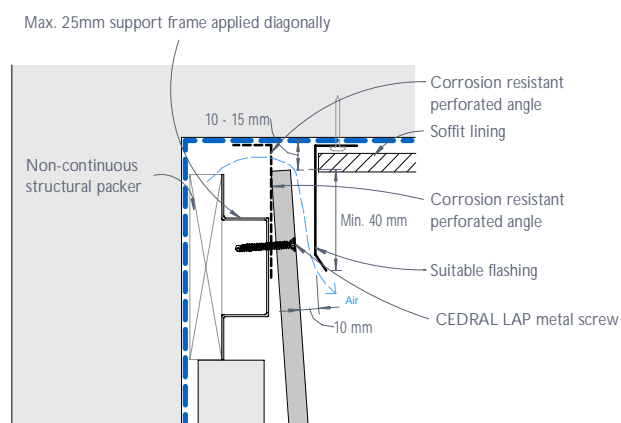
Figure 23: CEDRAL LAP junction with angled eave - Section A
