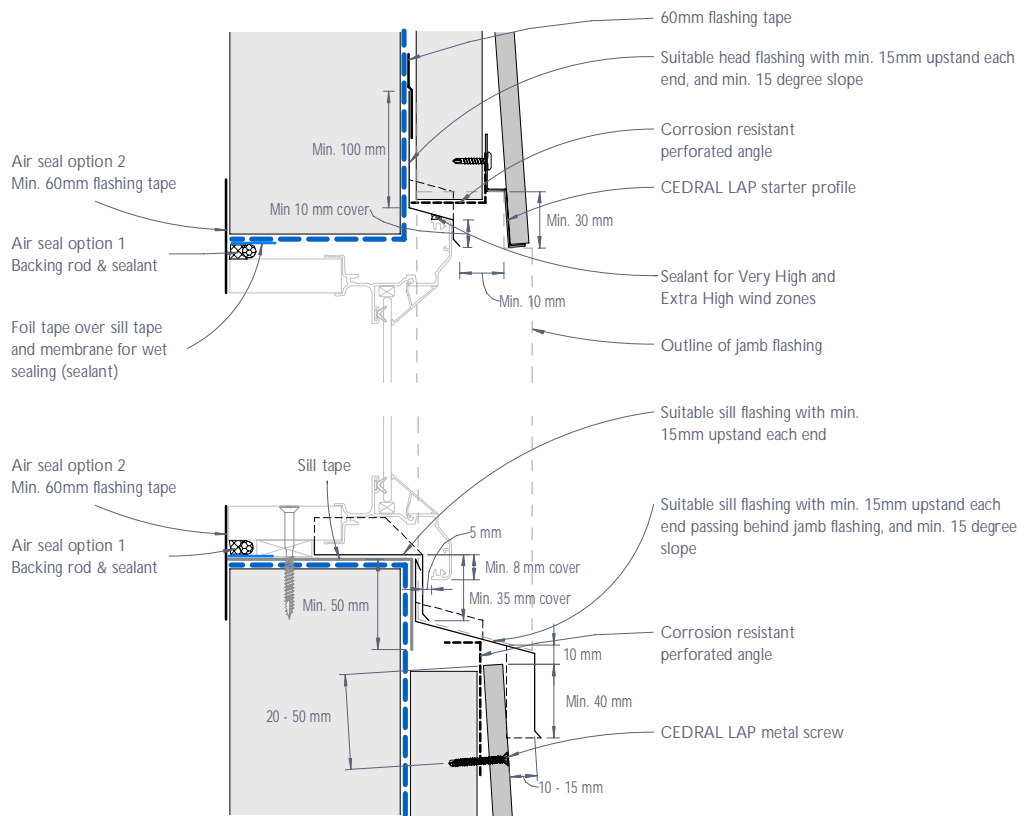
Figure 9: CEDRAL LAP window head and sill junction with CEDRAL starter profile at the head
