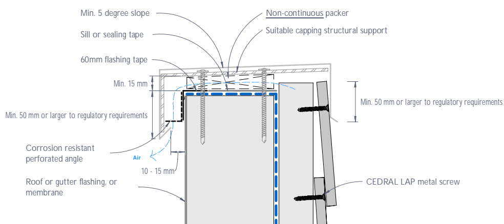
Figure 35: CEDRAL LAP flush capping detail
