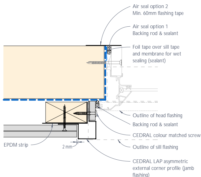
Figure 10: CEDRAL LAP window jamb junction or the like - Detail 1
