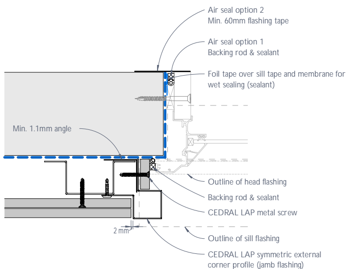
Figure 11: CEDRAL LAP window jamb junction or the like - Detail 2
