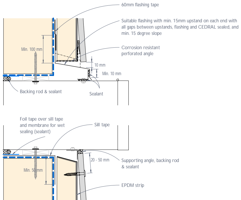
Figure 13: CEDRAL LAP meter box junction - Section
