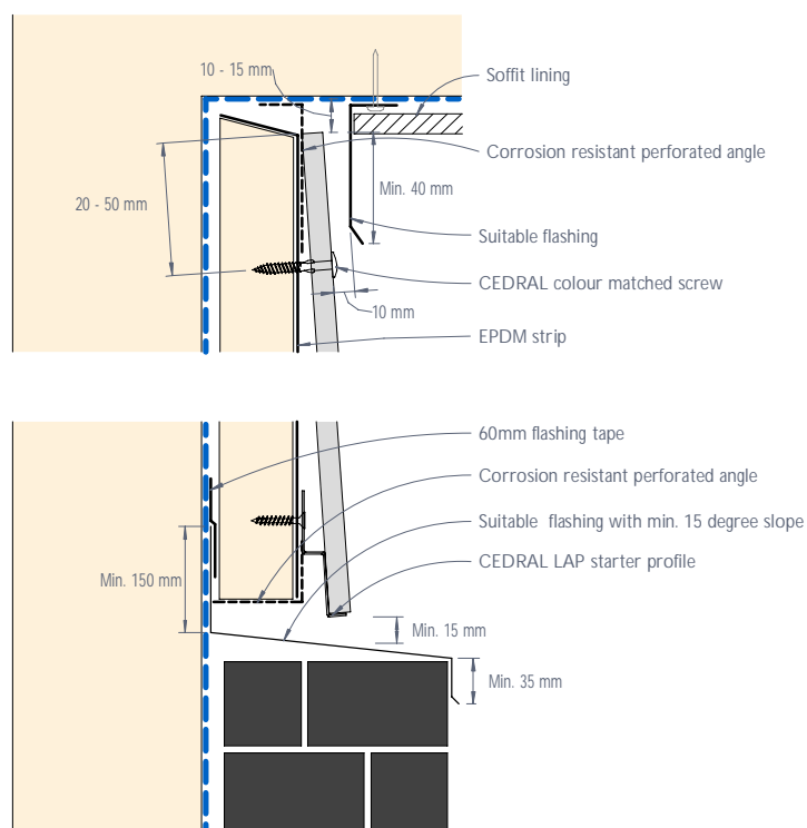
Figure 21: CEDRAL LAP junction with other materials, eaves or the like - Recessed detail
