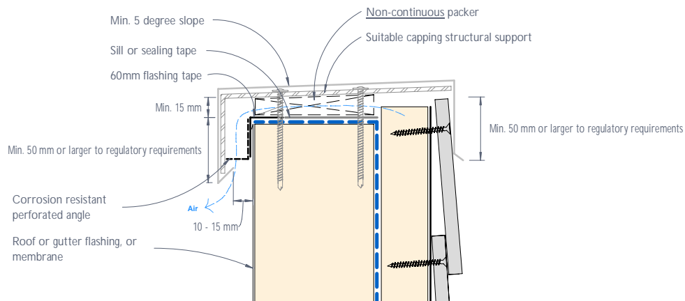
Figure 35: CEDRAL LAP flush capping detail
