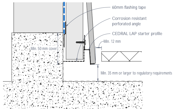
Figure 18: CEDRAL LAP base detail - Covered area
