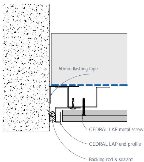
Figure 30: CEDRAL LAP abutment detail
