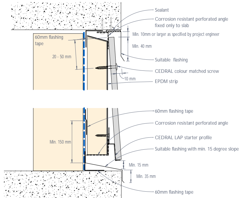
Figure 24: CEDRAL LAP junction with exposed concrete slab or beam - Cladding flush
