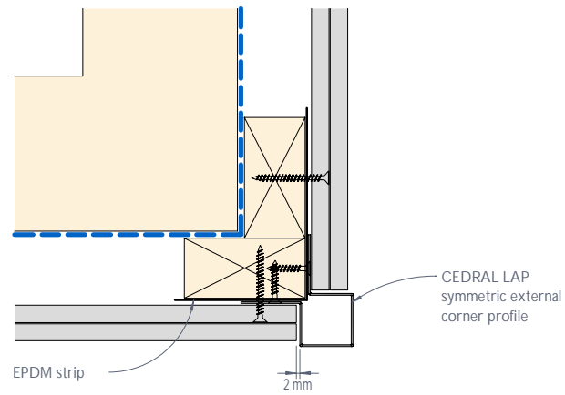
Figure 26: CEDRAL LAP typical external corner
