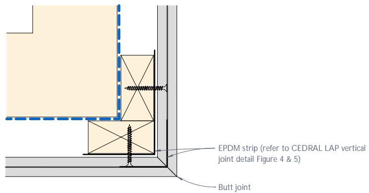
Figure 28: CEDRAL LAP mitered external corner
