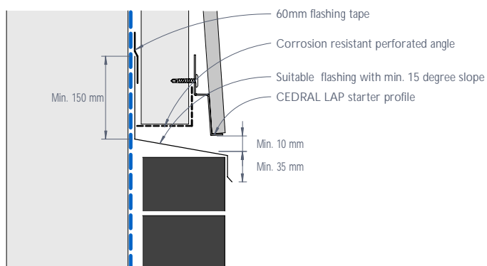
Figure 20: CEDRAL LAP junction with other materials - Flush detail
