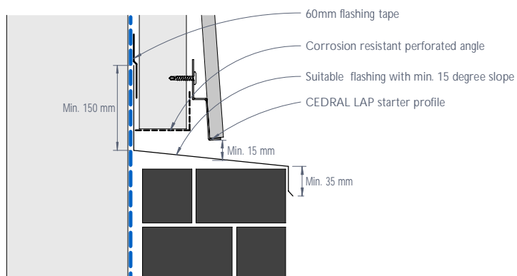
Figure 21: CEDRAL LAP junction with other materials, eaves or the like - Recessed detail
