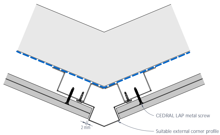
Figure 27: CEDRAL LAP 45 degree external corner
