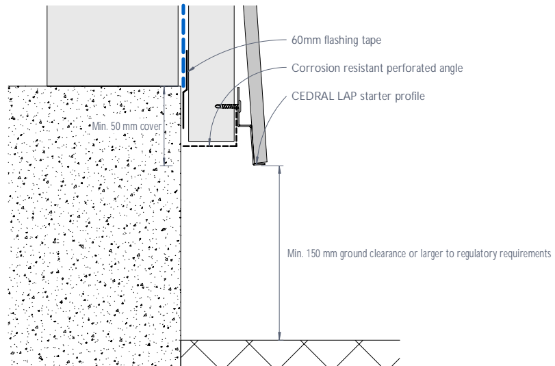
Figure 17: CEDRAL LAP base detail
