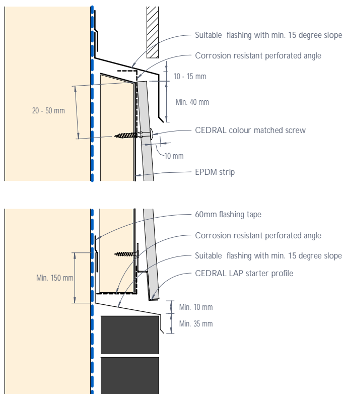
Figure 20: CEDRAL LAP junction with other materials - Flush detail
