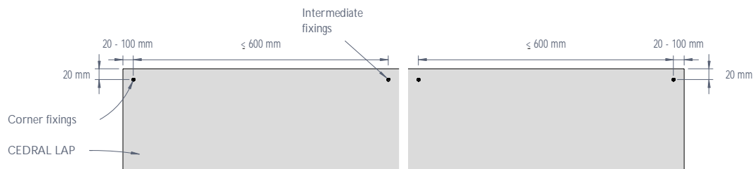
Figure 1: CEDRAL LAP fixings arrangement - Elevation
