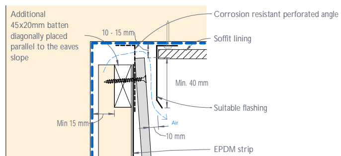
Figure 23: CEDRAL LAP junction with angled eave - Section A
