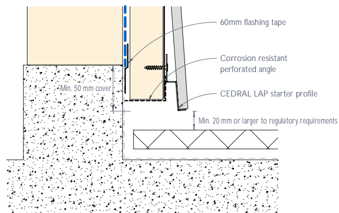
Figure 19: CEDRAL LAP base detail - Balcony
