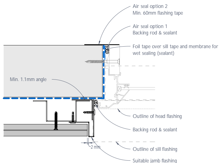
Figure 12: CEDRAL LAP window jamb junction or the like - Detail 3
