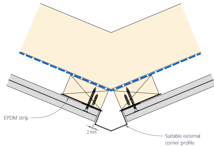
Figure 27: CEDRAL LAP 45 degree external corner
