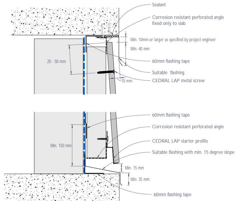
Figure 24: CEDRAL LAP junction with exposed concrete slab or beam - Cladding flush
