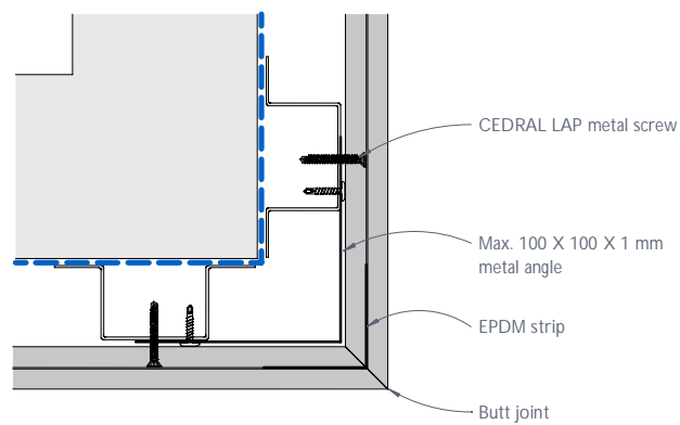
Figure 28: CEDRAL LAP mitered external corner
