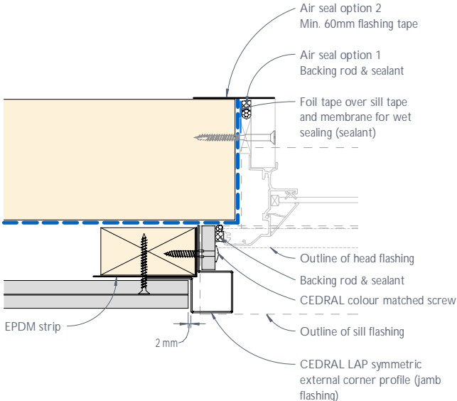
Figure 11: CEDRAL LAP window jamb junction or the like - Detail 2
