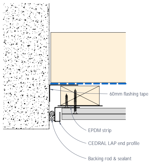
Figure 30: CEDRAL LAP abutment detail
