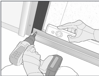
Ensure the starter profile is installed true level and next to the corner/end profiles
