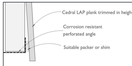
Planks trimmed in height should be packed out appropriately
