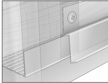
The starter profile is installed over the ventilated profile, and next to the vertical profile.
