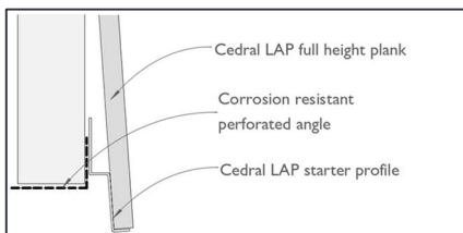
Cedral Lap starter profile is only used with full height plank
