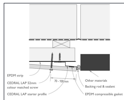
Cedral Lap Vertical – first plank – plan view
