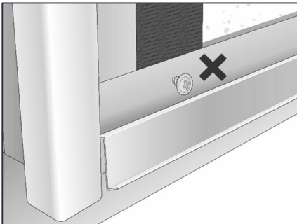
Use stainless steel low profile wafer head screws for fixing Cedral flashings and starter profiles to support frame. Ensure screws sit flush with the profile surface.
