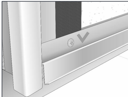
Use stainless steel low profile wafer head screws for fixing Cedral flashings and starter profiles to support frame. Ensure screws sit flush with the profile surface.
