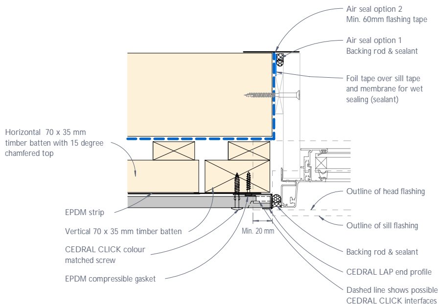
Figure 12: CEDRAL CLICK typical residential window jamb junction or the like - Flush detail
