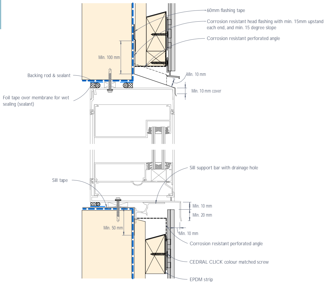
Figure 15: CEDRAL CLICK typical commercial window head and sill junction - Flush detail
