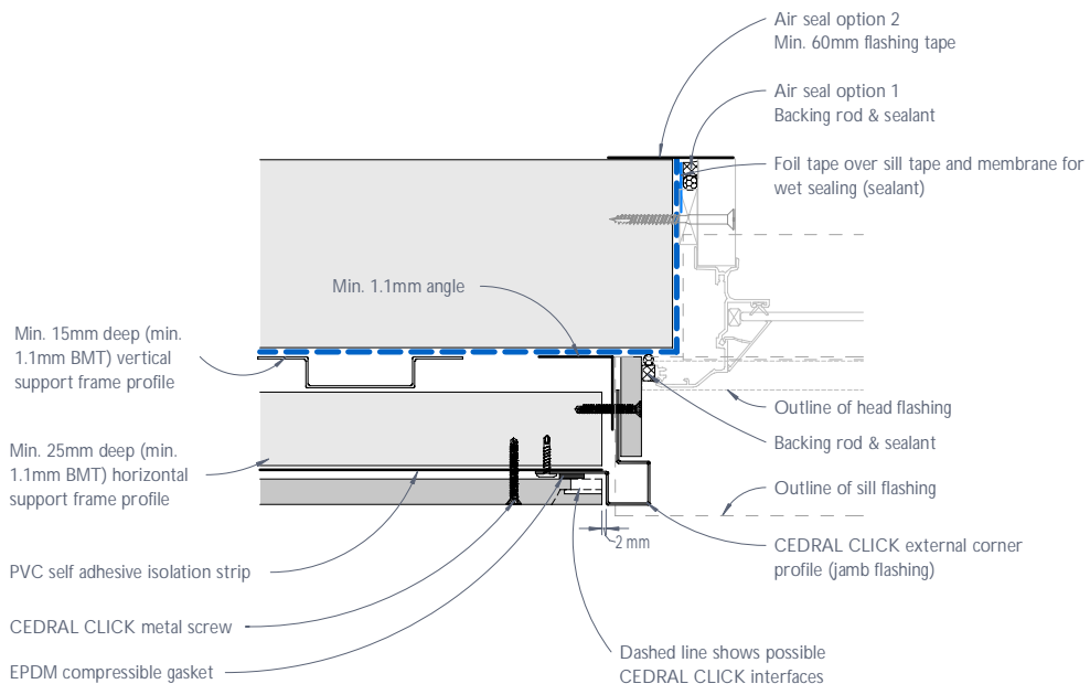
Figure 17: CEDRAL CLICK typical flange window jamb junction or the like - Recessed detail
