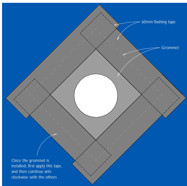
Figure 38: Pipe penetration - Elevation
