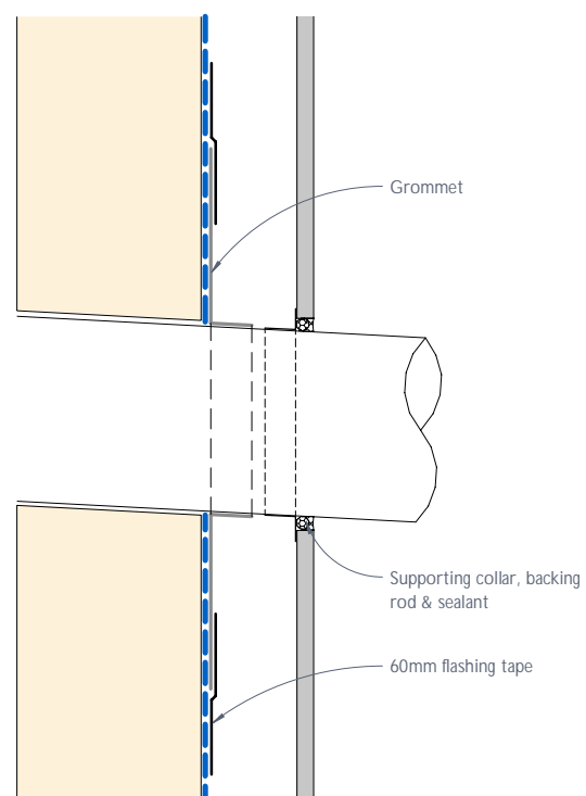
Figure 39: Pipe penetration - Section
