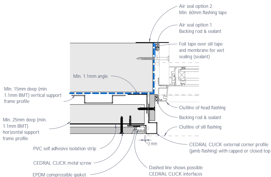
Figure 9: CEDRAL CLICK typical residential window jamb junction or the like - Recessed detail
