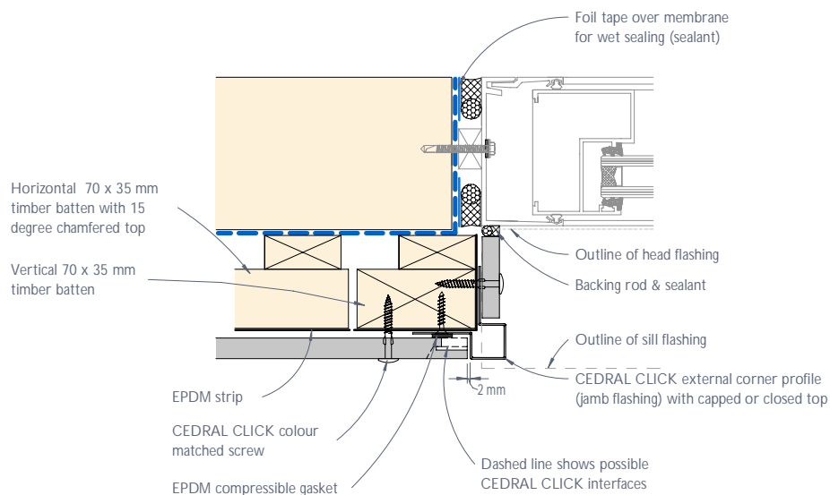
Figure 14: CEDRAL CLICK typical commercial window jamb junction or the like - Recessed detail
