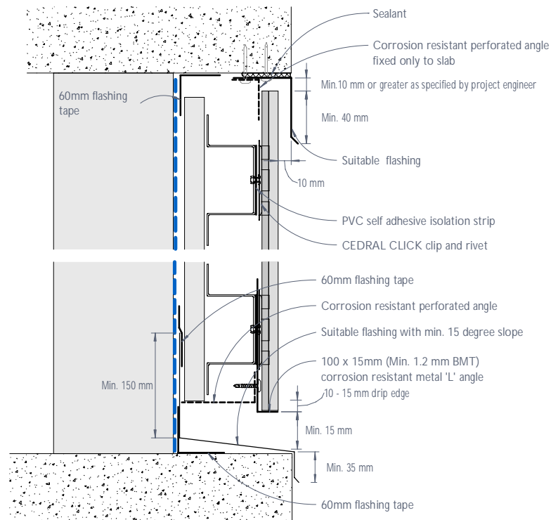
Figure 30: CEDRAL CLICK junction with exposed concrete slab or beam - Cladding flush
