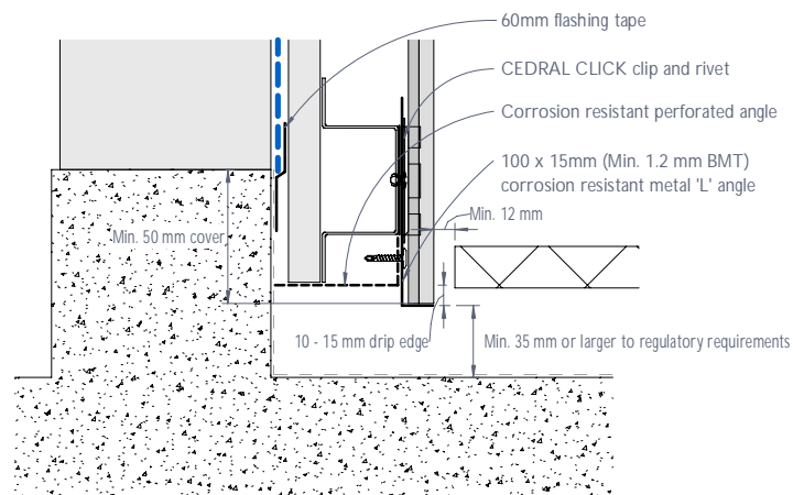
Figure 26: CEDRAL CLICK base detail - Covered area
