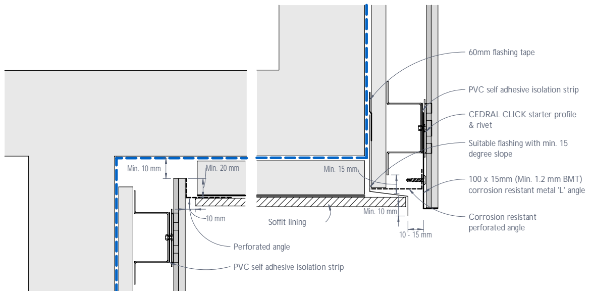
Figure 24: CEDRAL CLICK soffit junction
