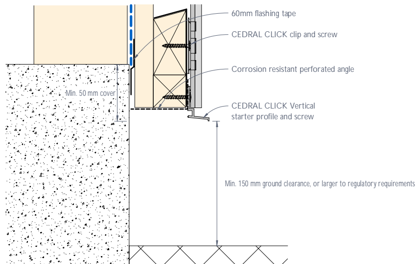
Figure 26: CEDRAL CLICK base detail
