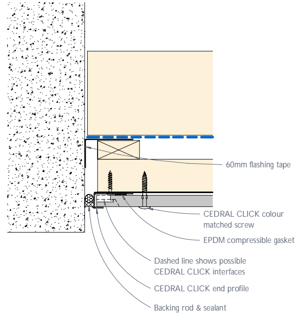
Figure 36: CEDRAL CLICK abutment detail
