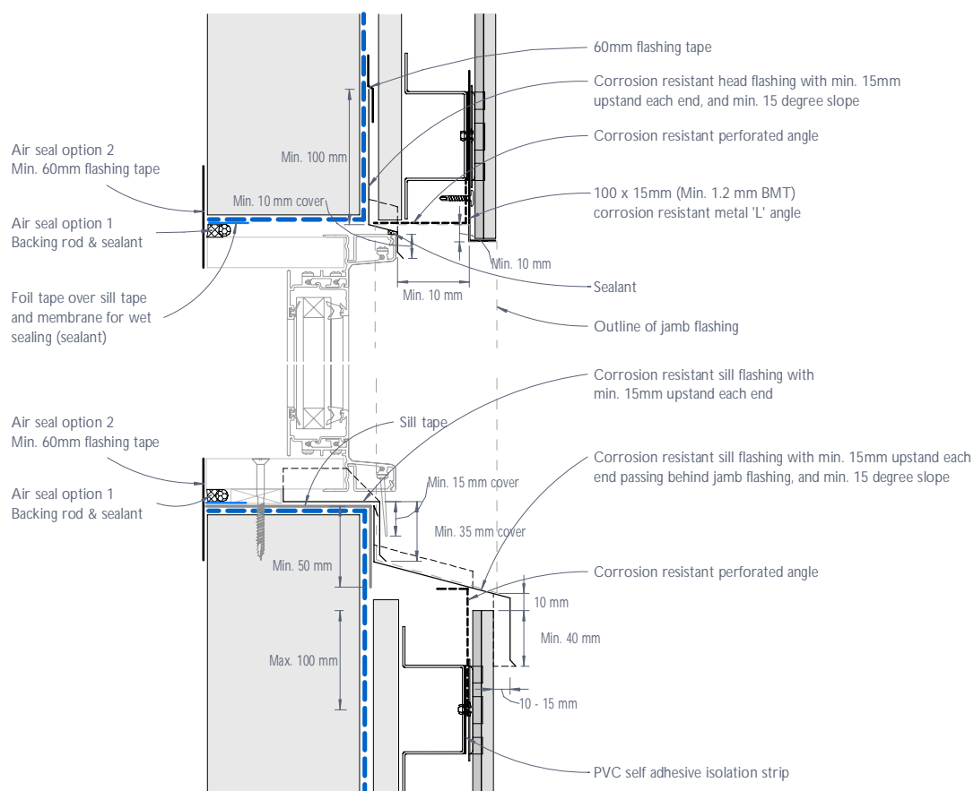
Figure 8: CEDRAL CLICK typical residential window head and sill junction - Recessed detail
