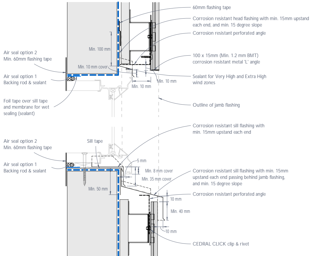
Figure 16: CEDRAL CLICK typical flange window head and sill junction or the like - Recessed detail
