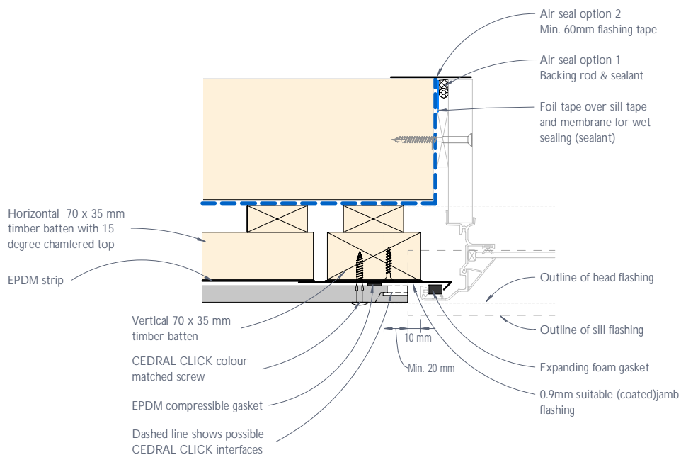
Figure 20: CEDRAL CLICK typical flange window jamb junction or the like - Flush detail
