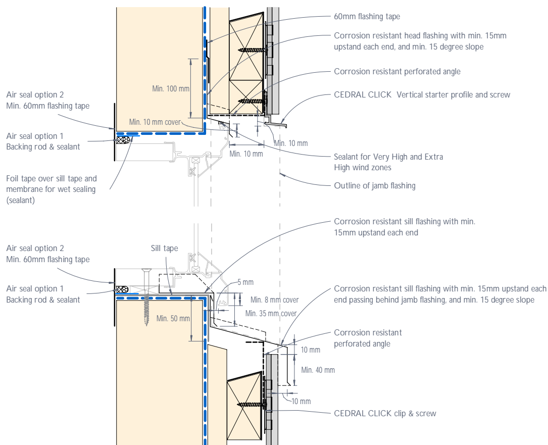
Figure 17: CEDRAL CLICK typical flange window head and sill junction or the like - Recessed detail
