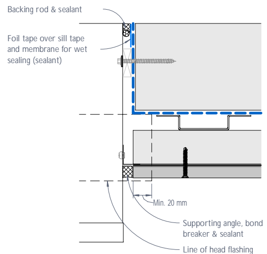
Figure 22: CEDRAL CLICK meter box junction Plan view - Option 2
