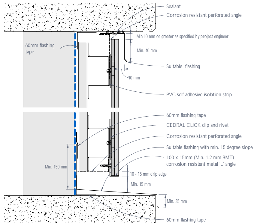
Figure 31: CEDRAL CLICK junction with exposed concrete slab or beam - Cladding recessed
