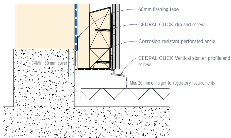
Figure 28: CEDRAL CLICK base detail - Balcony
