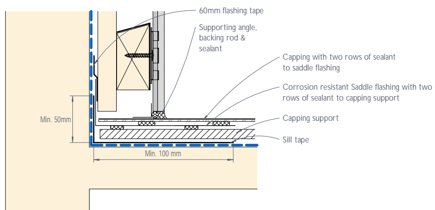
Figure 42: CEDRAL CLICK parapet junction - Section
