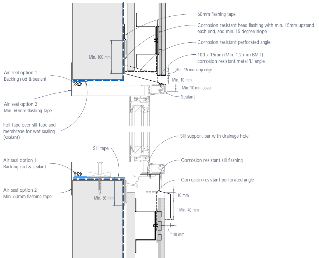
Figure 10: CEDRAL CLICK typical residential window head and sill junction or the like - Flush detail
