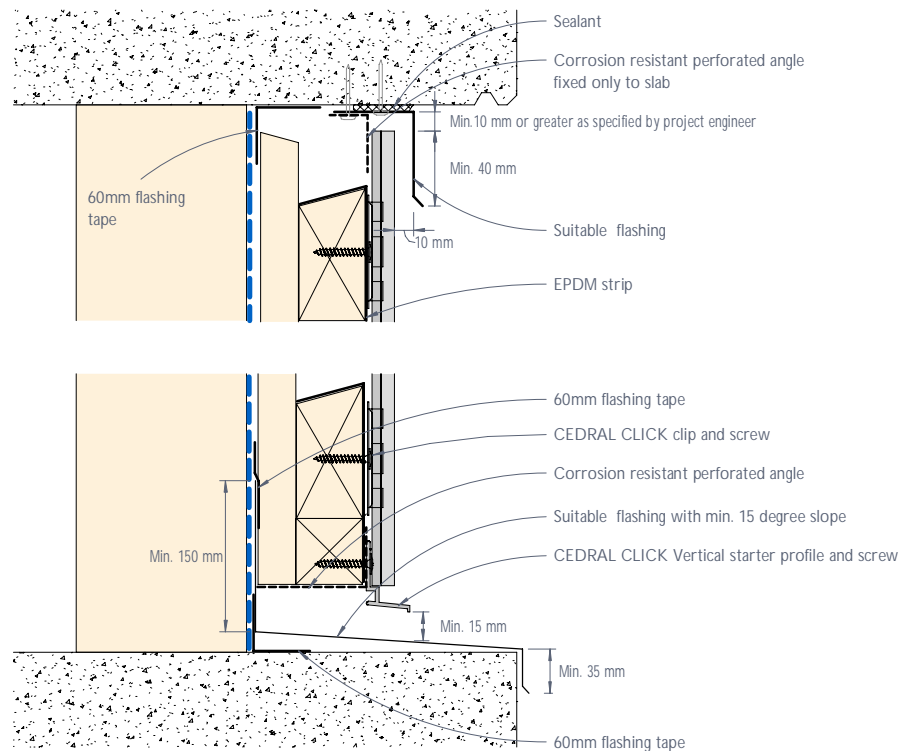
Figure 32: CEDRAL CLICK junction with exposed concrete slab or beam - Cladding recessed
