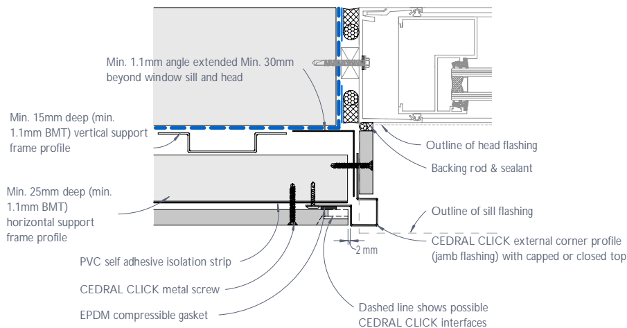
Figure 13: CEDRAL CLICK typical commercial window jamb junction or the like - Recessed detail
