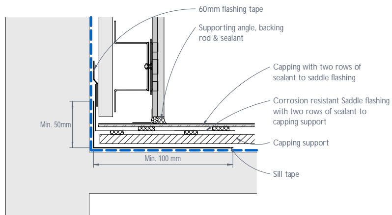
Figure 41: CEDRAL CLICK parapet junction - Section
