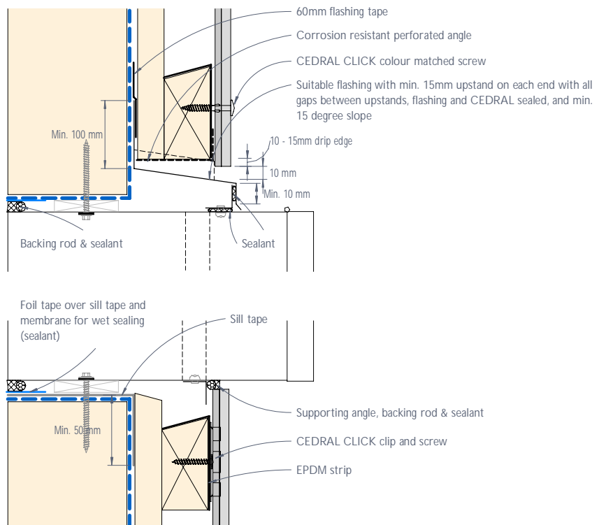
Figure 21: CEDRAL CLICK meter box junction - Section
