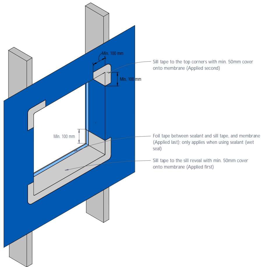
Figure 23: Isometric view of window/meter box opening - Tape application
