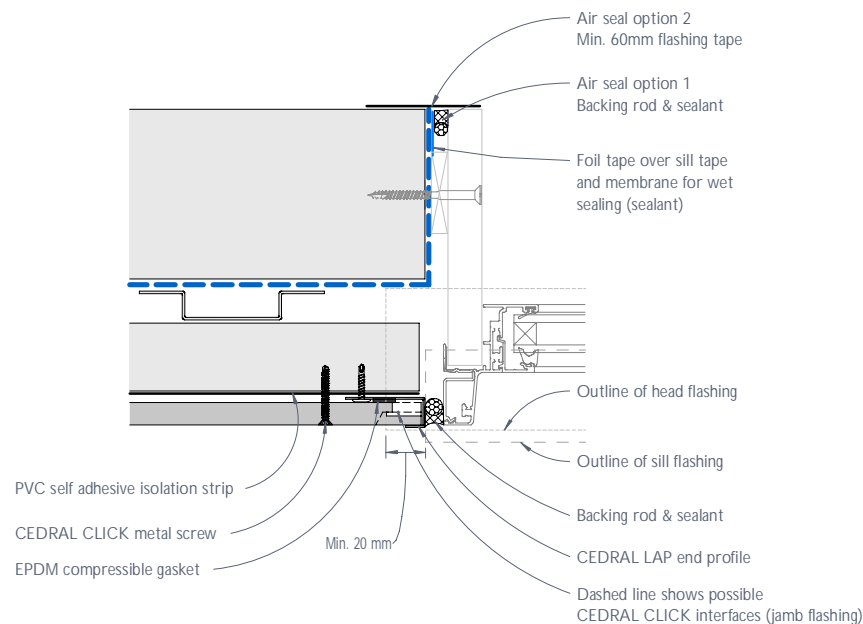
Figure 11: CEDRAL CLICK typical residential window jamb junction or the like - Flush detail
