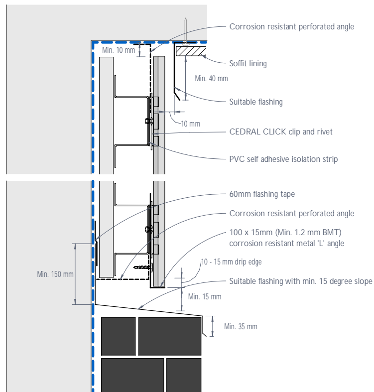
Figure 29: CEDRAL CLICK junction with other materials, eaves or the like - Recessed detail
