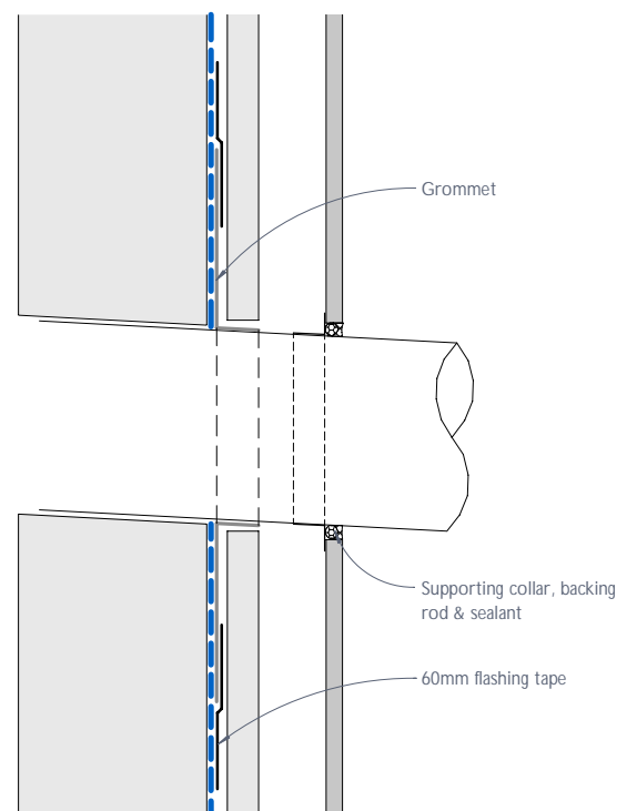
Figure 38: Pipe penetration - Section
