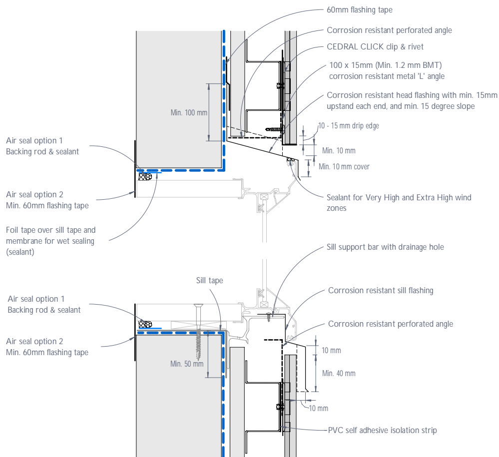
Figure 18: CEDRAL CLICK typical flange window head and sill junction - Flush detail
