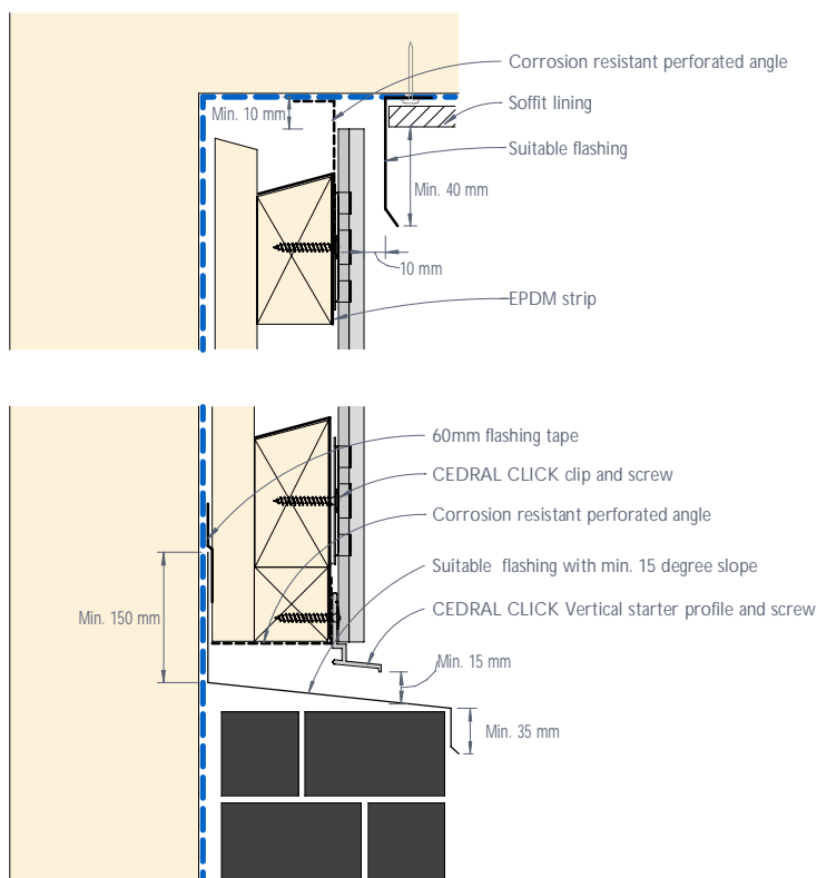
Figure 30: CEDRAL CLICK junction with other materials, eaves or the like - Recessed detail
