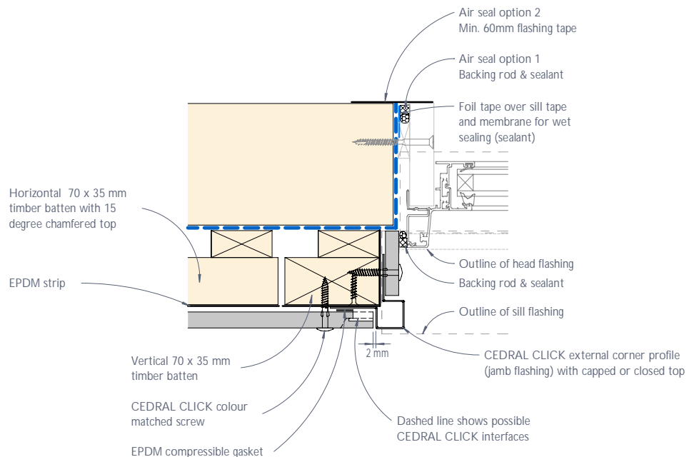
Figure 10: CEDRAL CLICK typical residential window jamb junction or the like - Recessed detail
