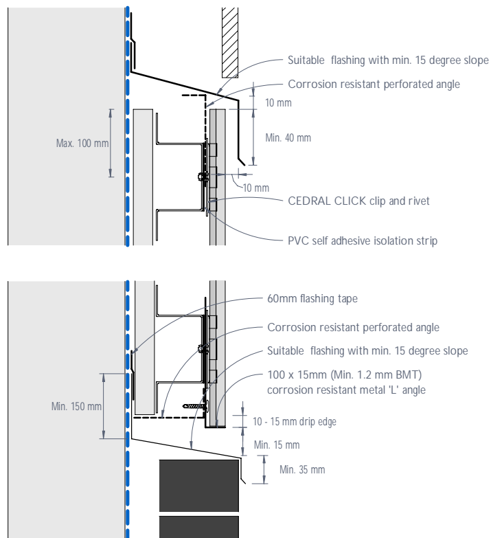
Figure 28: CEDRAL CLICK junction with other materials - Flush detail
