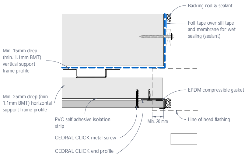
Figure 21: CEDRAL CLICK meter box junction Plan view - Option 1
