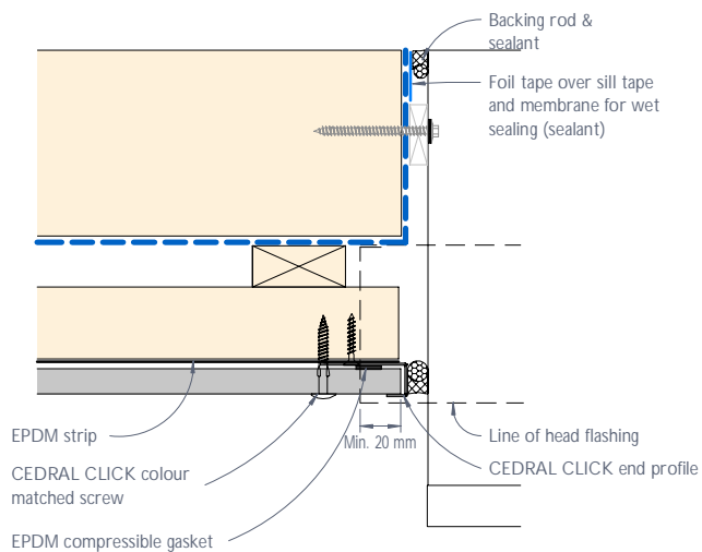
Figure 22: CEDRAL CLICK meter box junction Plan view - Option 1
