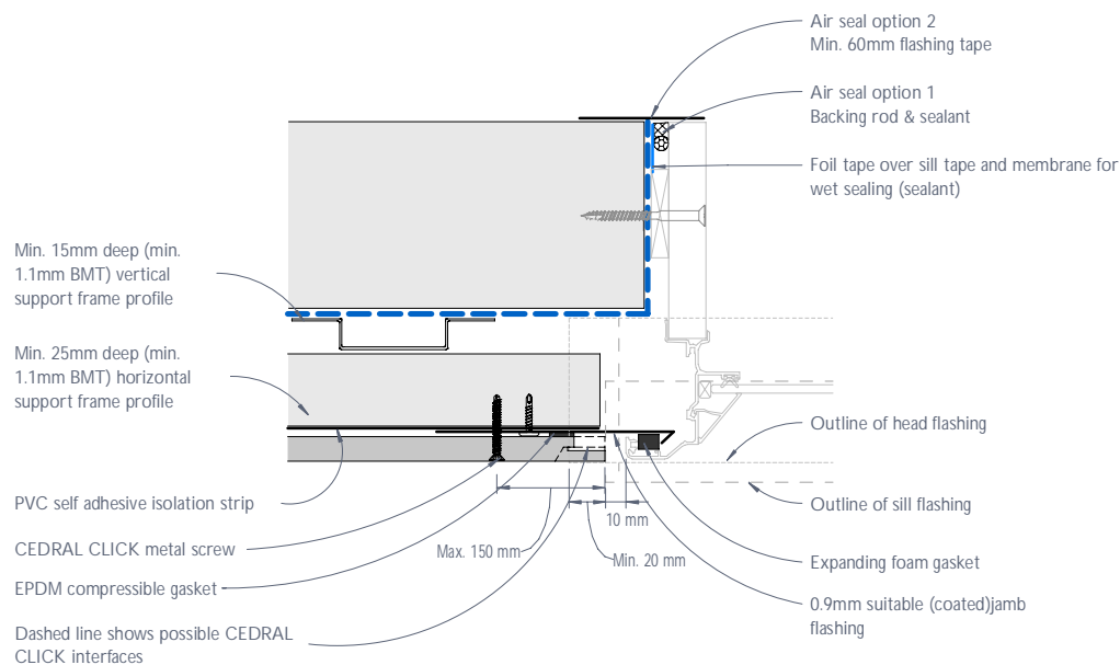
Figure 19: CEDRAL CLICK typical flange window jamb junction or the like - Flush detail
