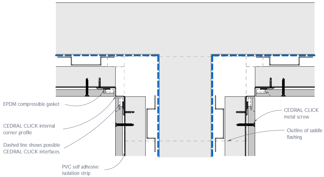
Figure 42: Parapet junction - Plan view
