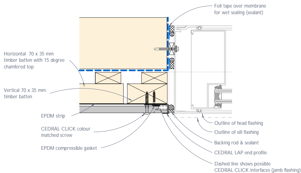
Figure 16: CEDRAL CLICK typical commercial window jamb junction or the like - Flush detail
