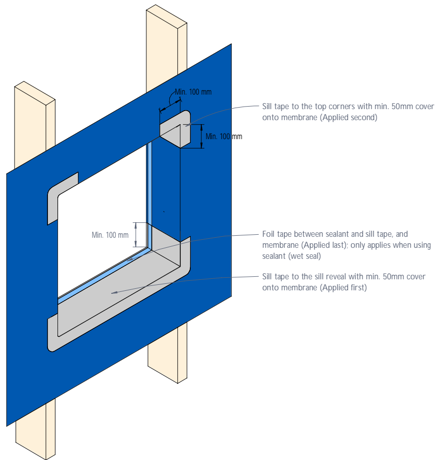
Figure 24: Isometric view of window/meter box opening - Tape application
