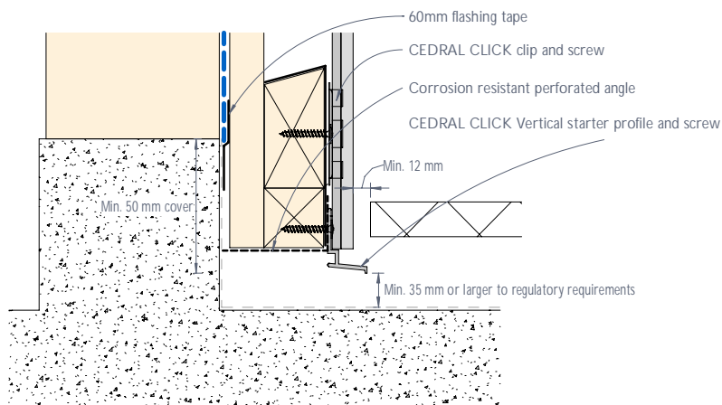
Figure 27: CEDRAL CLICK base detail - Covered area
