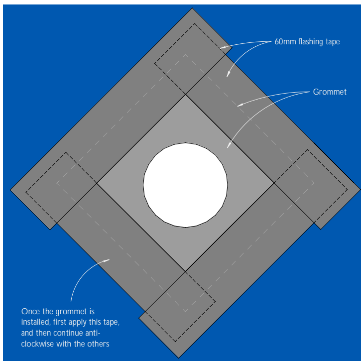
Figure 37: Pipe penetration - Elevation
