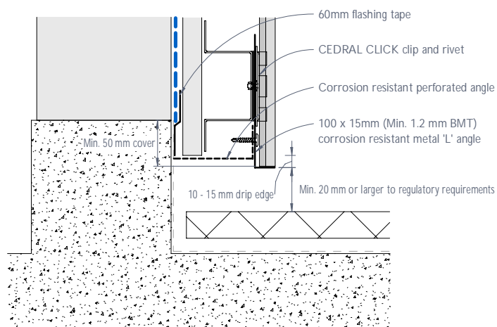
Figure 27: CEDRAL CLICK base detail - Balcony
