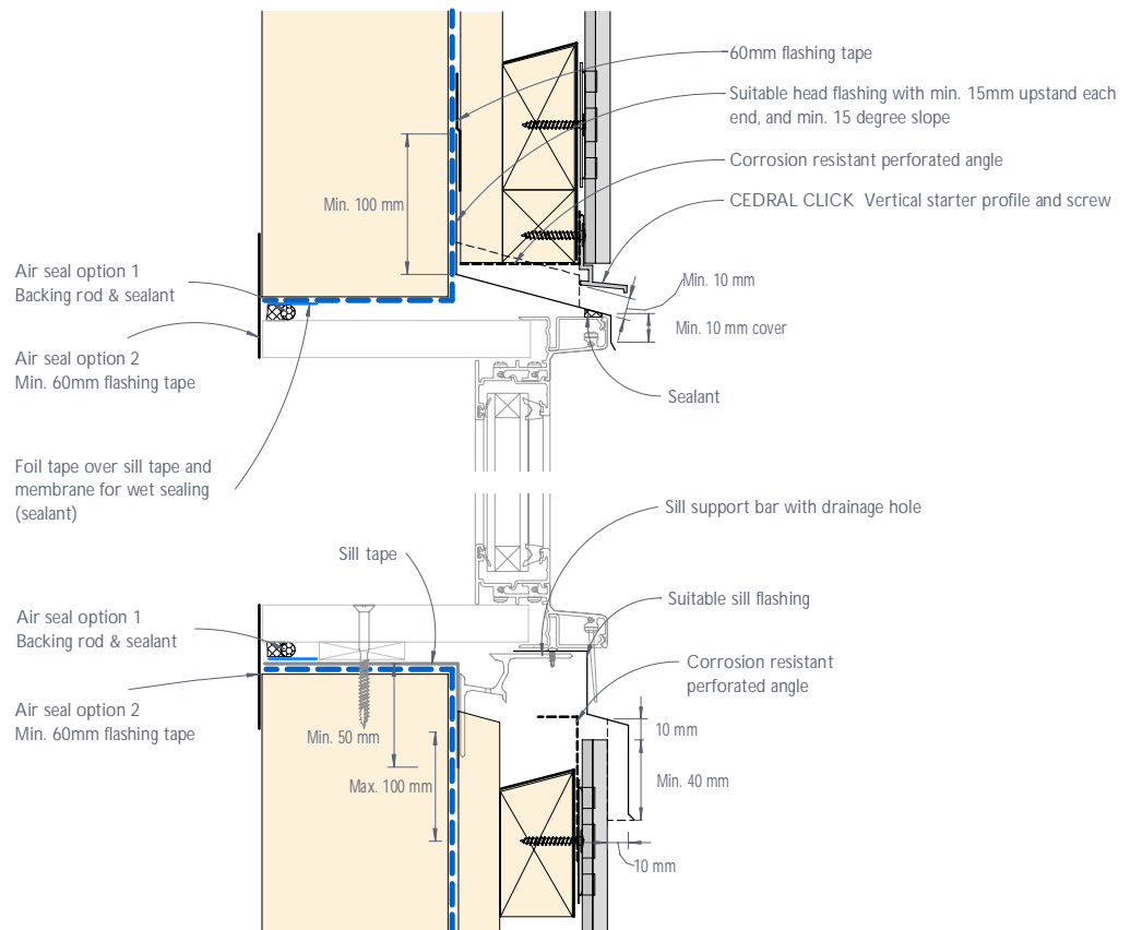
Figure 11: CEDRAL CLICK typical residential window head and sill junction or the like - Flush detail
