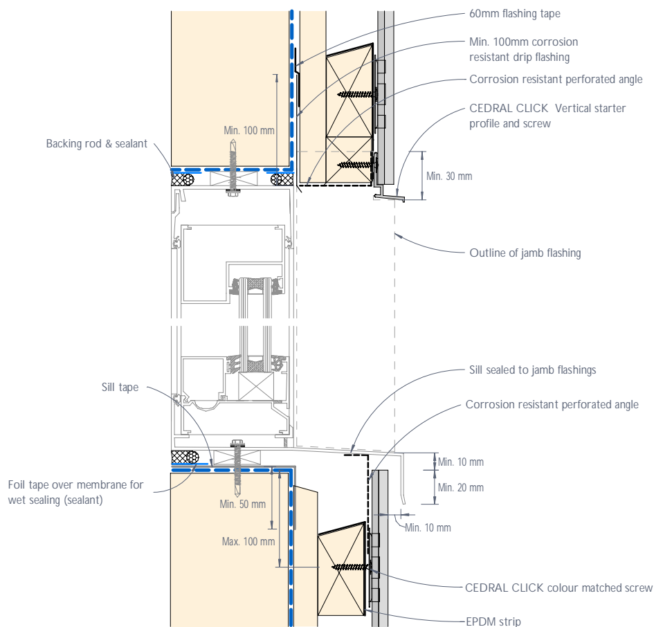
Figure 13: CEDRAL CLICK typical commercial window head and sill junction - Recessed detail
