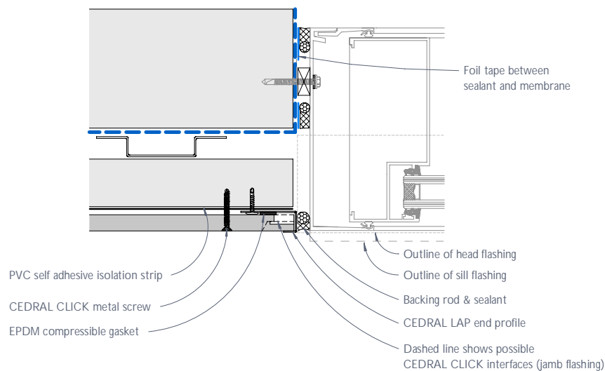
Figure 15: CEDRAL CLICK typical commercial window jamb junction or the like - Flush detail
