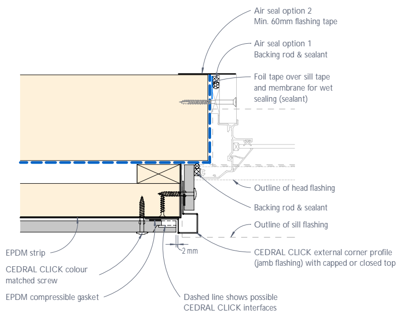
Figure 18: CEDRAL CLICK typical flange window jamb junction or the like - Recessed detail
