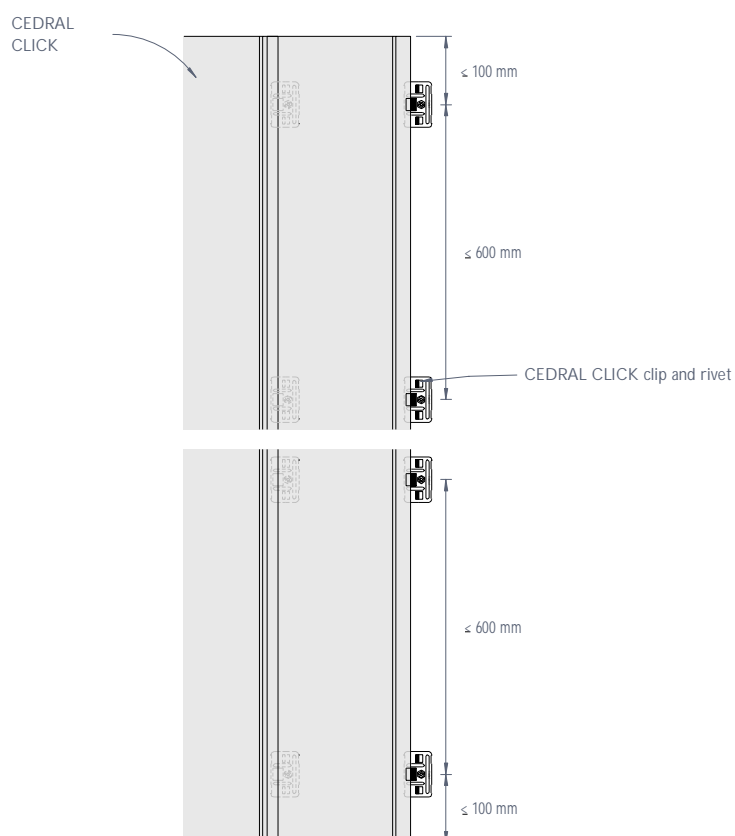
Figure 1: CEDRAL CLICK fixings arrangement - Elevation
