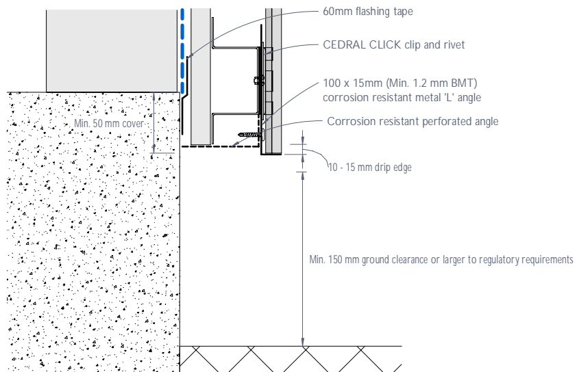
Figure 25: CEDRAL CLICK base detail
