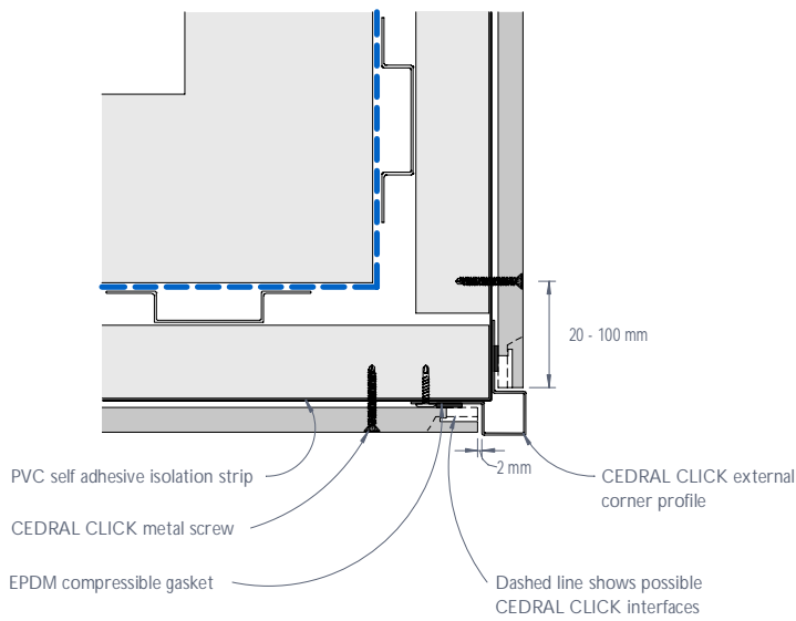
Figure 32: CEDRAL CLICK typical external corner
