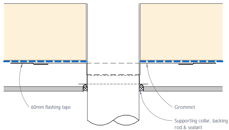
Figure 37: Pipe penetration - Plan view
