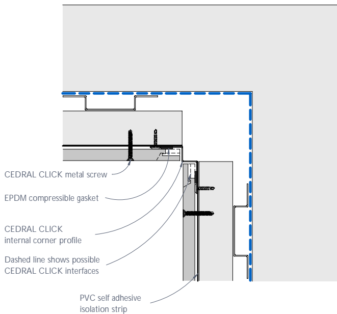
Figure 34: CEDRAL CLICK internal corner
