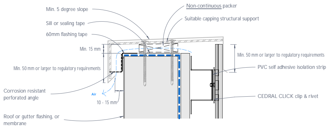
Figure 40: CEDRAL CLICK flush capping detail
