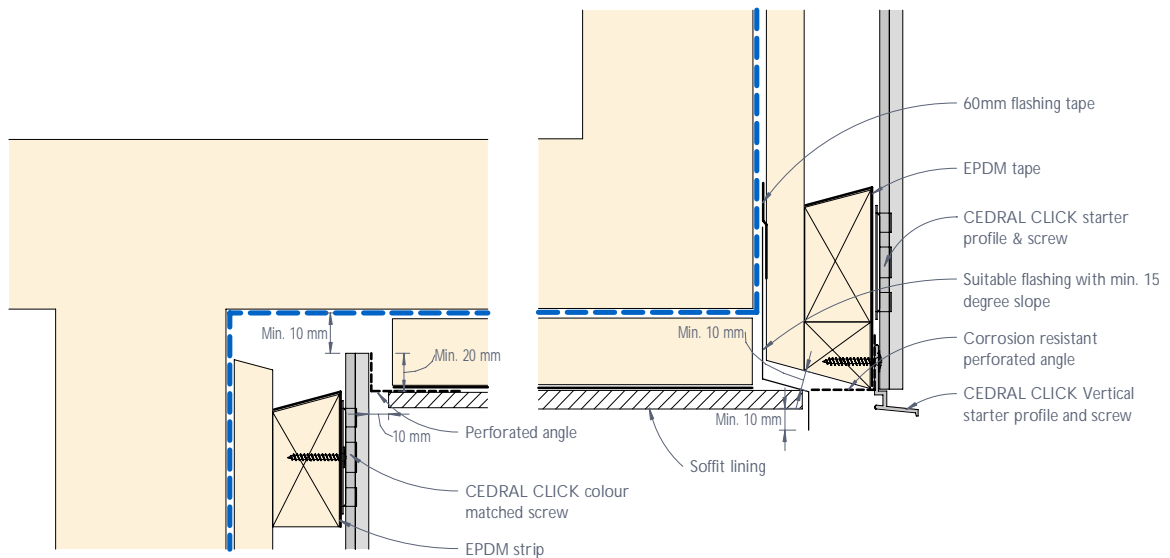
Figure 25 CEDRAL CLICK soffit junction
