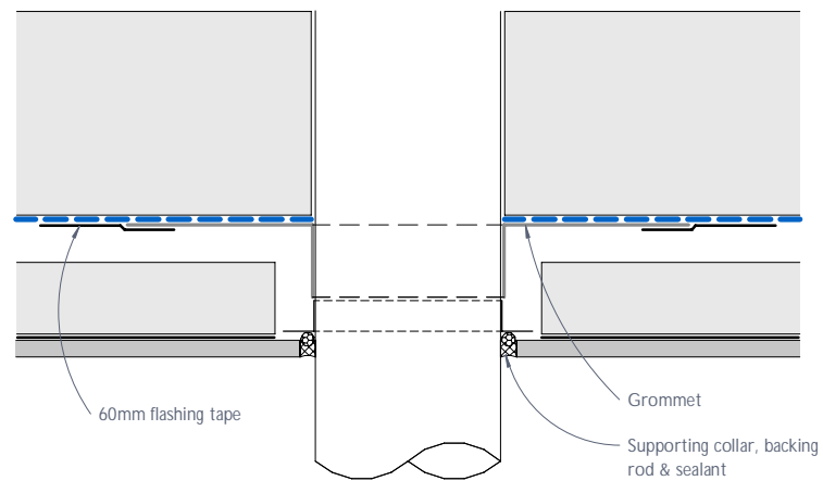
Figure 36: Pipe penetration - Plan view
