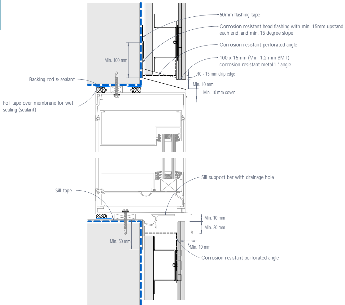
Figure 14: CEDRAL CLICK typical commercial window head and sill junction - Flush detail
