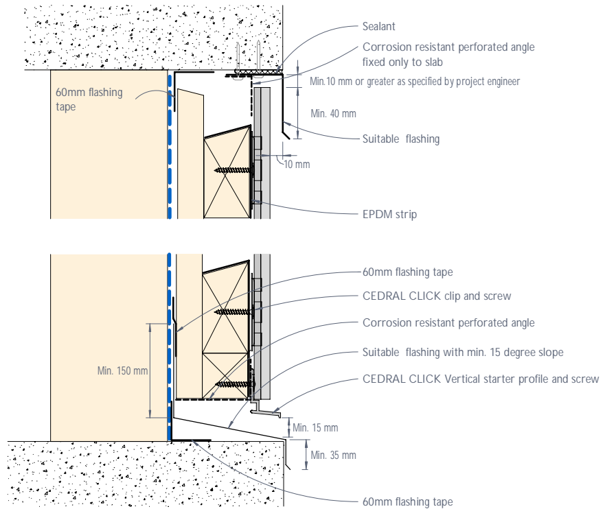
Figure 31: CEDRAL CLICK junction with exposed concrete slab or beam - Cladding flush
