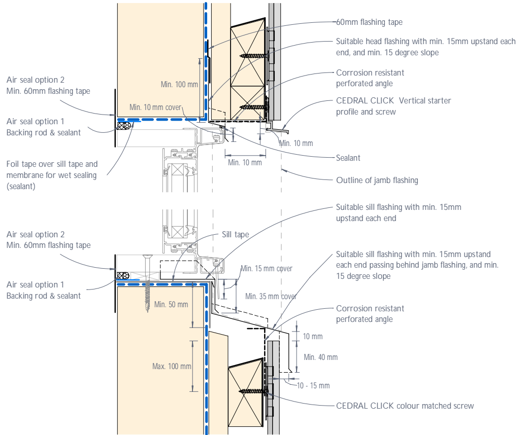
Figure 9: CEDRAL CLICK typical residential window head and sill junction - Recessed detail
