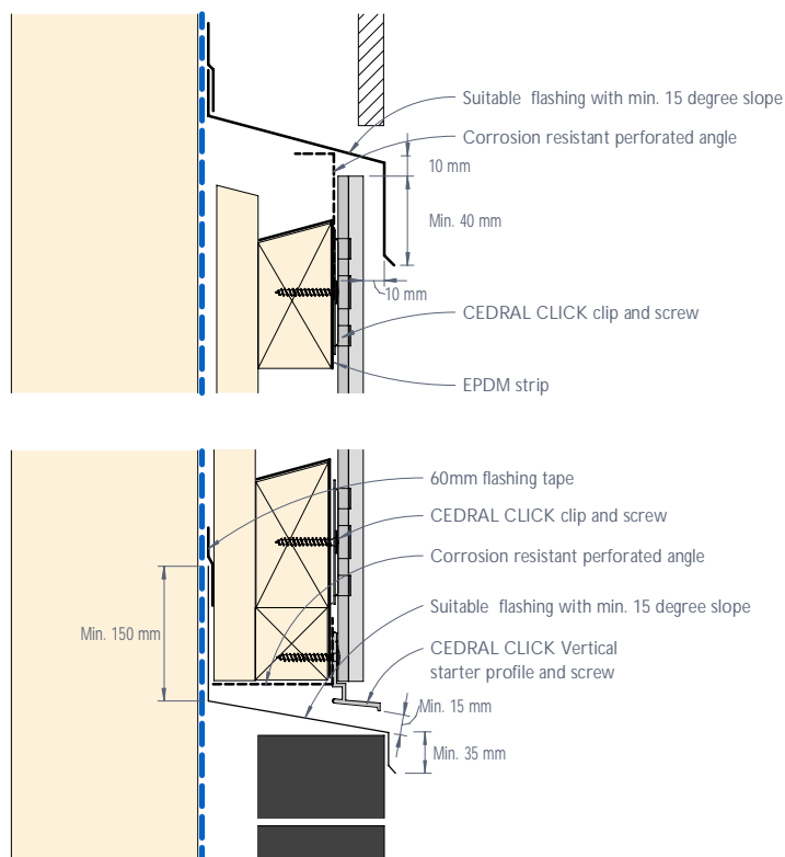
Figure 29: CEDRAL CLICK junction with other materials - Flush detail
