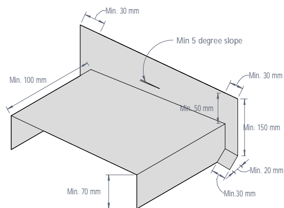
Figure 44: Corrosion resistant saddle flashing
