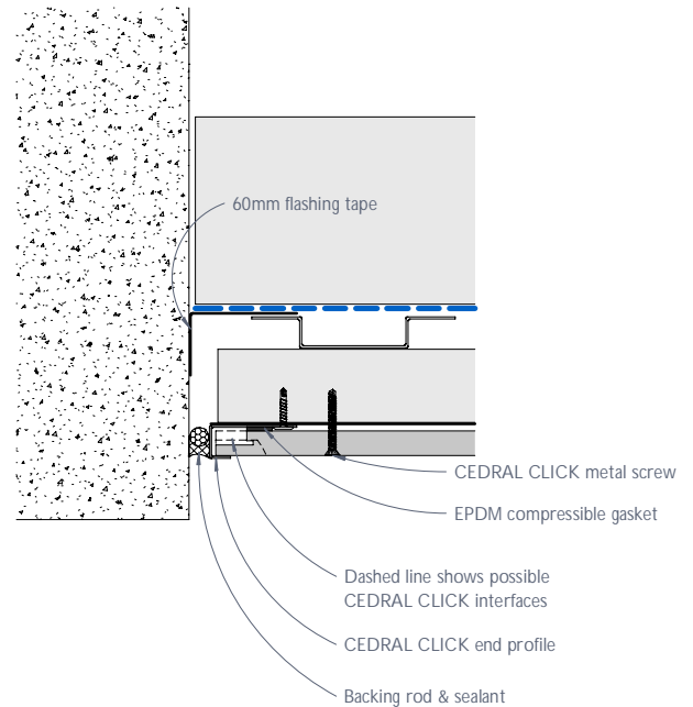
Figure 35: CEDRAL CLICK abutment detail
