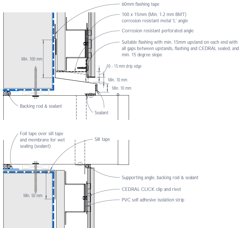
Figure 20: CEDRAL CLICK meter box junction - Section
