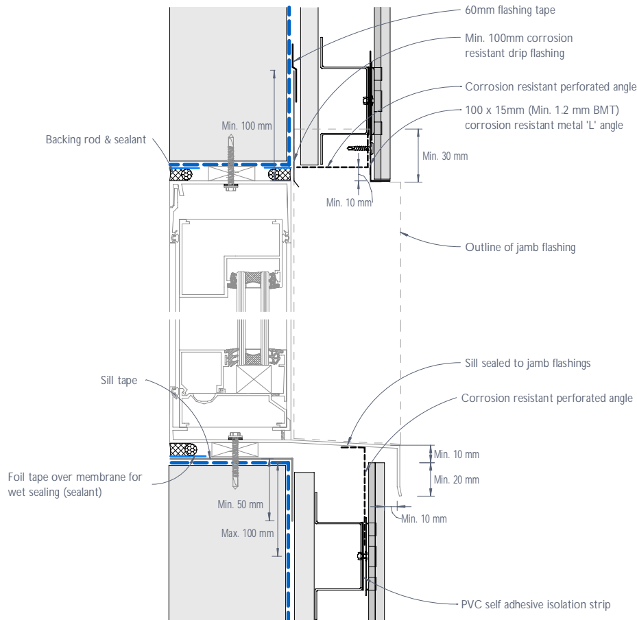
Figure 12: CEDRAL CLICK typical commercial window head and sill junction - Recessed detail
