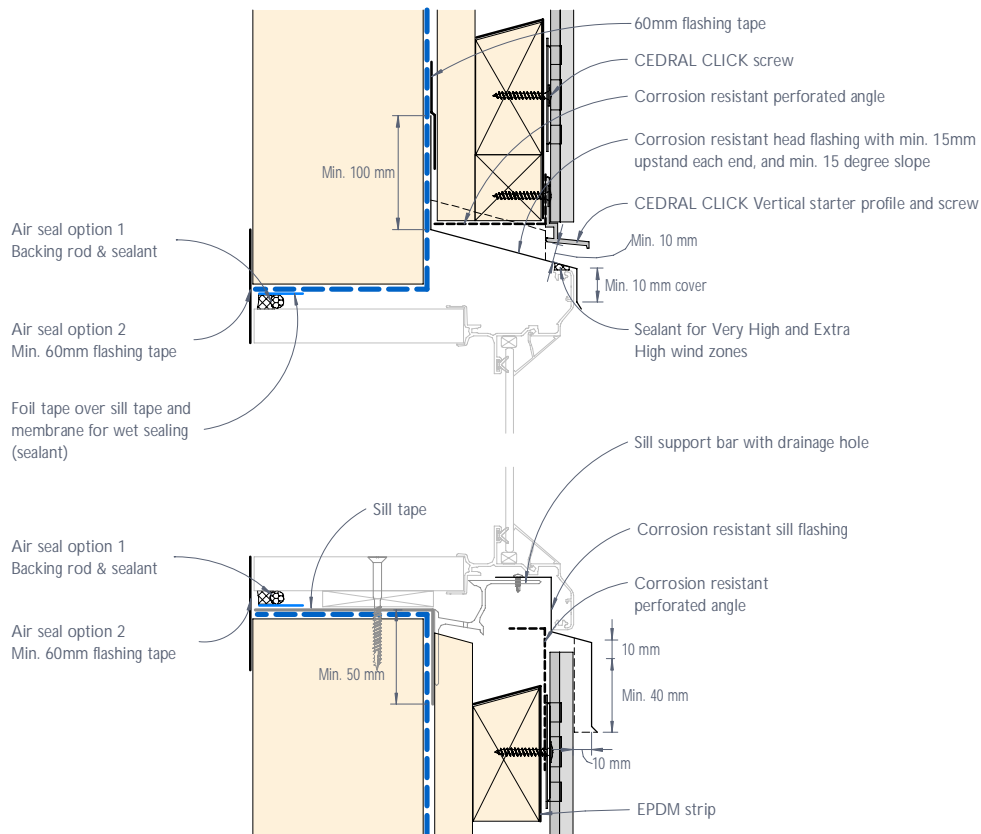
Figure 19: CEDRAL CLICK typical flange window head and sill junction - Flush detail
